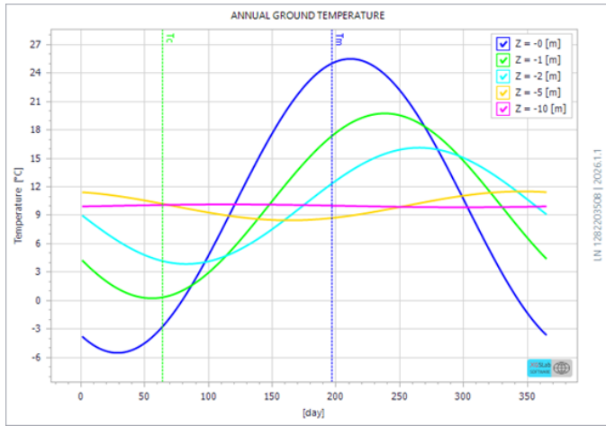
Annual ground temperature
