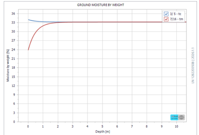
Ground moisture by weight as a function of depth
