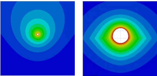
Electric Field (left) and Magnetic Field (right) at 1 MHz
