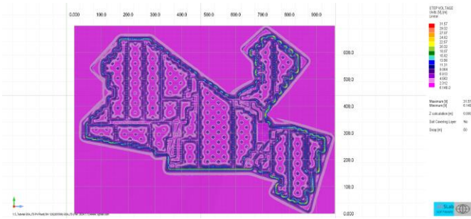
Step voltage - PV plant – Colors option
