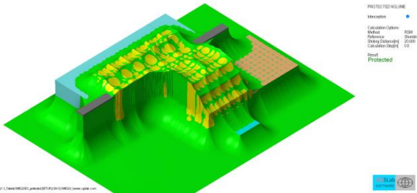
Protected Volume represented using a safety margin 5 m
