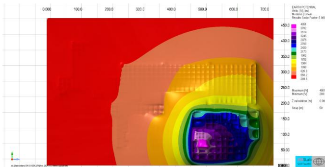
Earth surface potential - Large factory - Colors option
