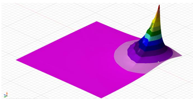
Earth surface potential - 100 kHz
