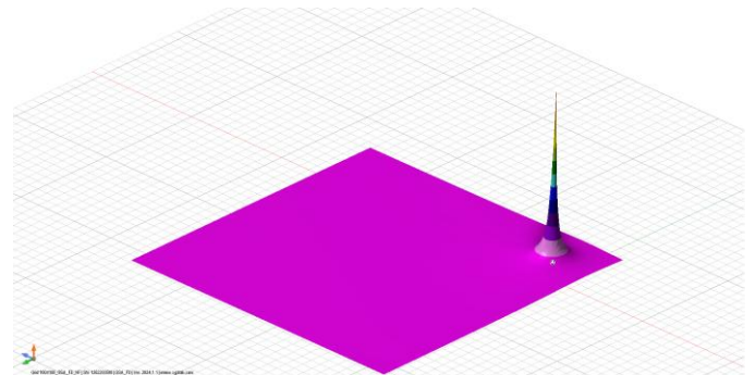
Earth surface potential - 100 MHz
