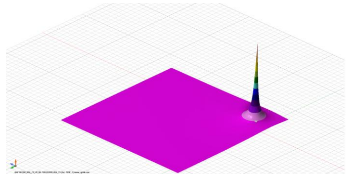
Earth surface potential - 10 MHz
