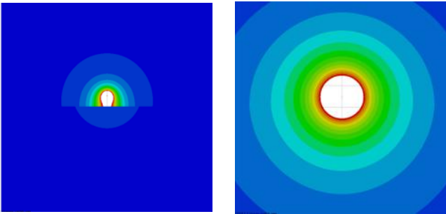
Electric Field (left) and Magnetic Field (right) at 10 kHz
