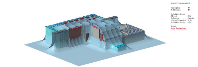
Protected Volume calculated with the Rolling Sphere method – Hydro Power Plant
