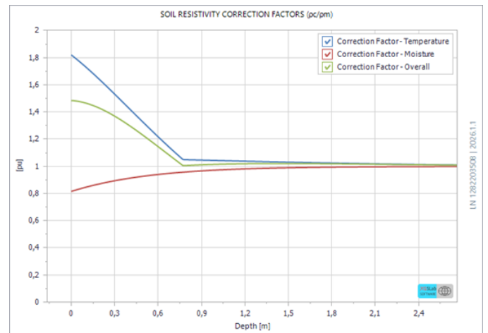
Soil resistivity correction factors as a function of depth
