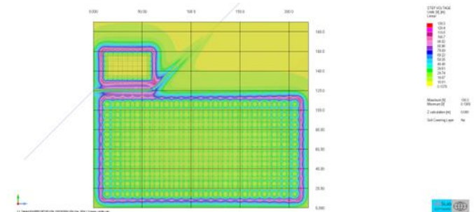
Step voltages - Factory - Colors option
