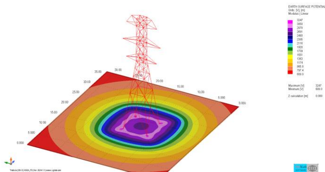
Earth surface potential – HV lattice – Colors option
