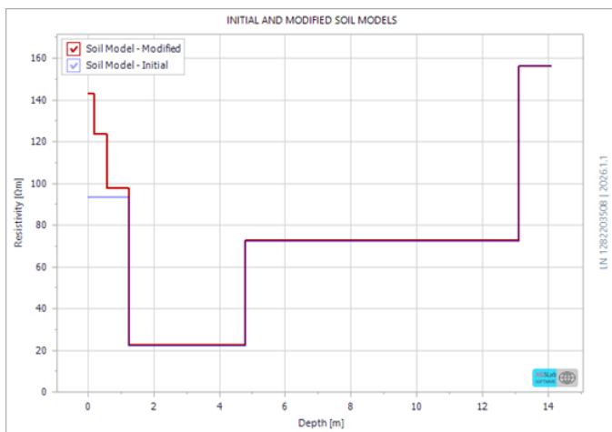
Initial and Modified Soil Models
