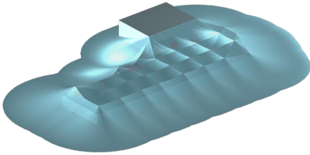
Protected Volume calculated with the Rolling Sphere method – Industrial plant
