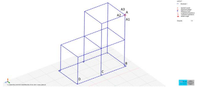
Building LPS and lightning current injection point
