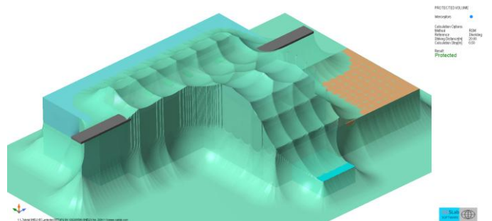
Protected Volume calculated with the Rolling Sphere method – Hydro Power Plant
