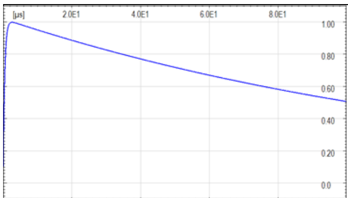
Normalized subsequent negative standard lightning - Linear scale
