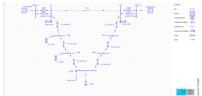
Network layout
