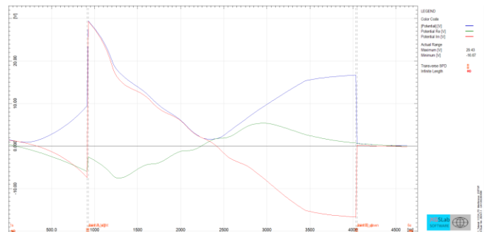
Induced potential on the pipeline (blue magnitude, green real, red imaginary)
