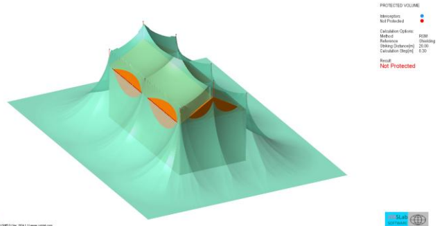
Protected Volume calculated with the Rolling Sphere method – Simple case
