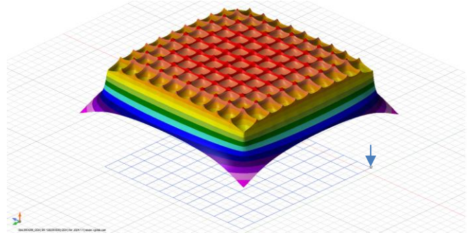
Earth surface potential - GSA or GSA_FD with high soil resistivity
