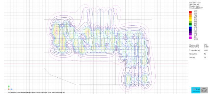
Electric field on horizontal surface - Substation - Contours option
