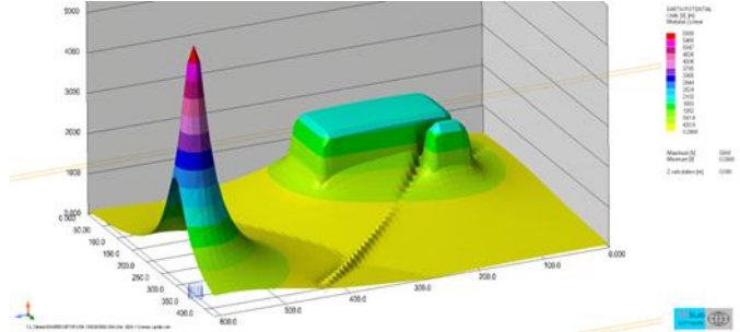
Earth surface potential - Factory – Colors option
