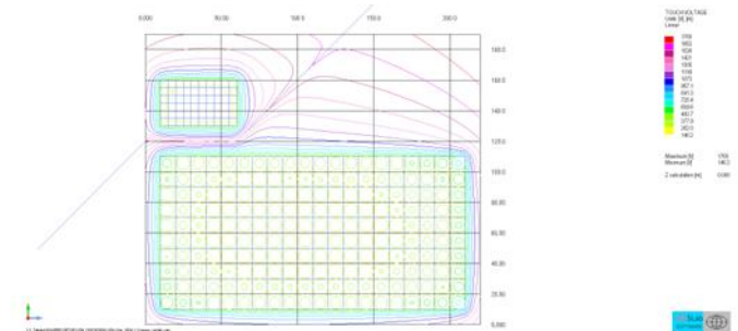
Touch voltages - Factory - Contours option
