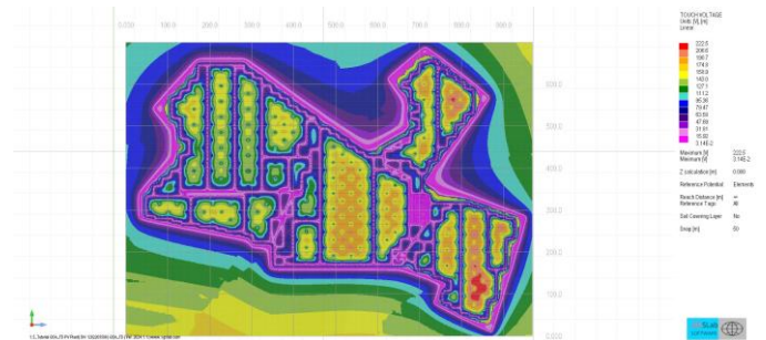
Touch voltage - PV plant - Colors option
