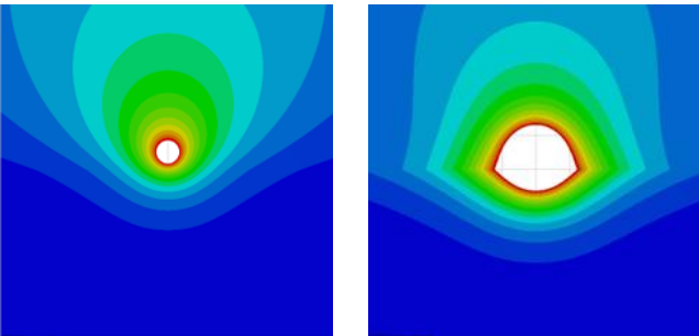
Electric Field (left) and Magnetic Field (right) at 10 MHz
