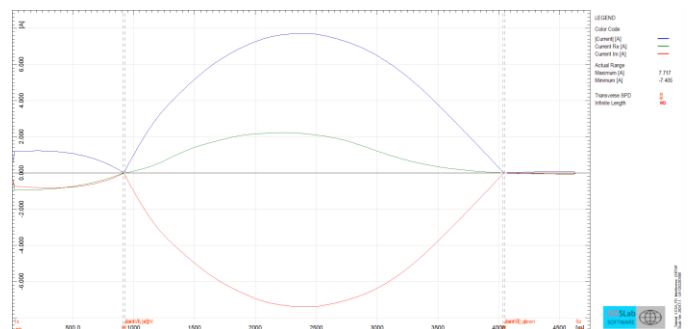
Induced current on the pipeline (blue magnitude, green real, red imaginary)
