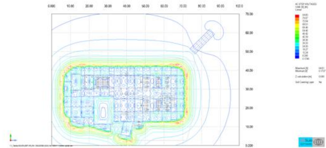
Step voltages – Substation - Contours option
