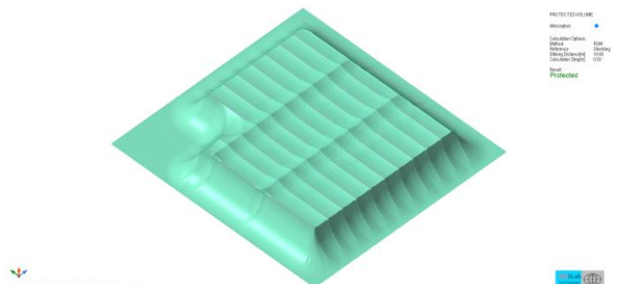
Protected Volume calculated with the Rolling Sphere method – Substation
