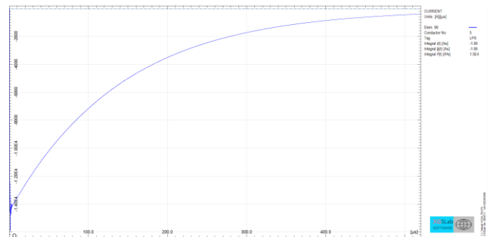
Current in the time domain in an air termination conductor (Linear scale)
