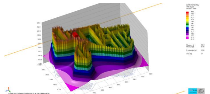
Earth surface potential - PV plant - Colors option
