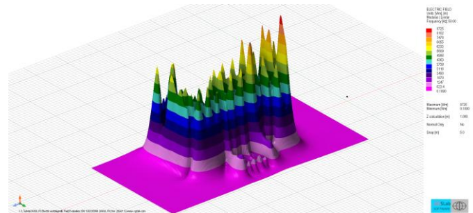
Electric field on an horizontal surface - Substation - Colors option
