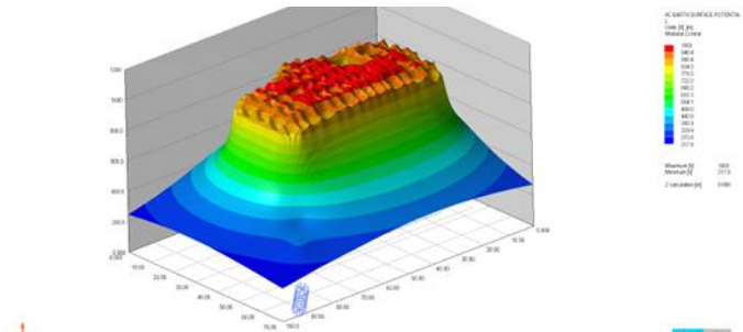
Earth surface potential - Substation - Colors option
