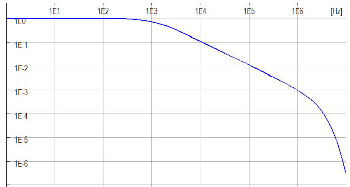
Normalized magnitude spectrum - Log scale
