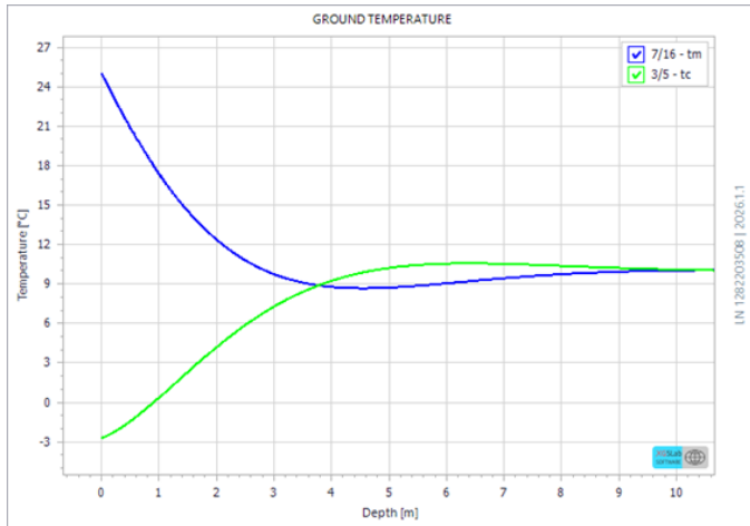
Ground temperature as a function of depth
