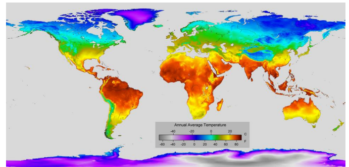
Annual average temperature World map
