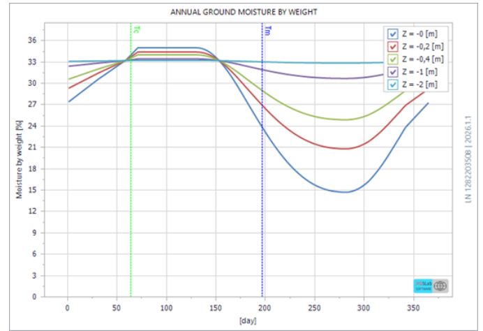
Annual ground moisture by weight
