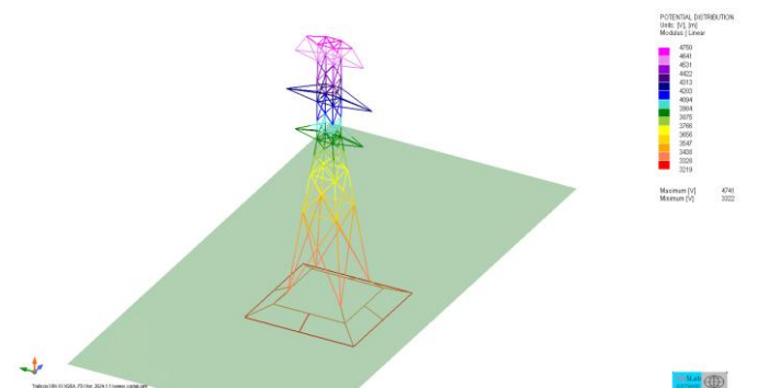
Potential - HV lattice
