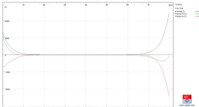
Potential along an OHEW - Magnitude, real and imaginary parts
