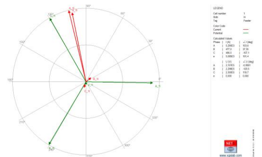
Phasor diagram (or Fresnel diagram) of potentials and currents at a cell side
