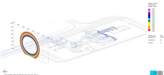
Magnetic field on vertical surface – Substation – Colors option
