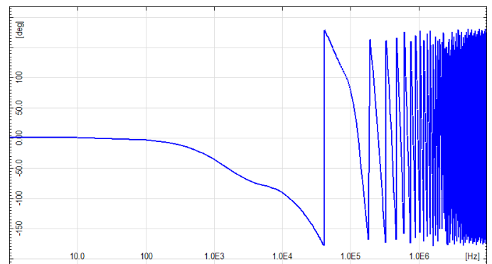
Normalized phase spectrum - Log Linear scale
