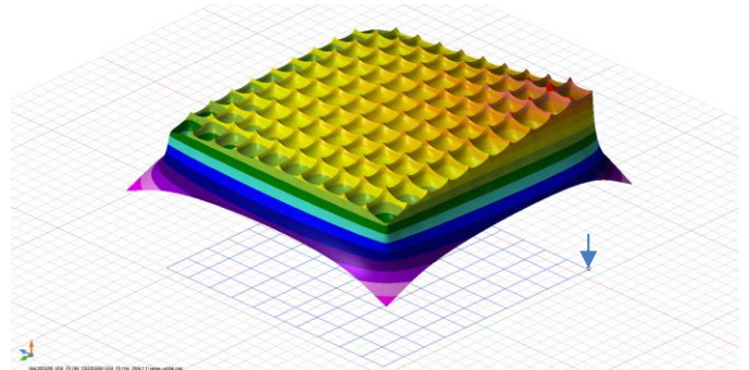
Earth surface potential - GSA_FD with medium soil resistivity
