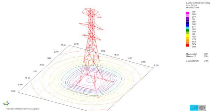
Earth surface potential – HV lattice – Contours option
