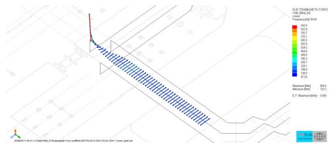
Electromagnetic force along conductors - Substation
