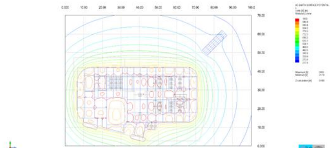
Earth surface potential - Substation - Contours option
