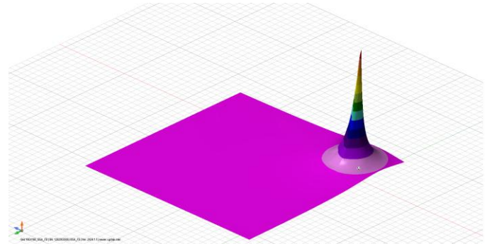
Earth surface potential - 1 MHz
