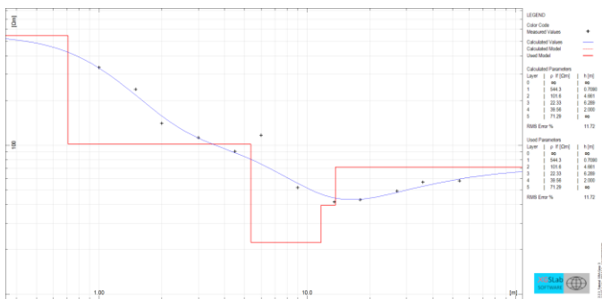
Soil resistivity measures and parameters of a five layers soil model - Log scale
