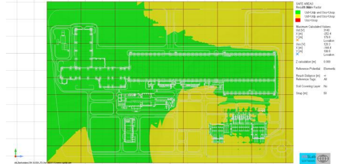
Touch and step voltages safe areas - Large factory
