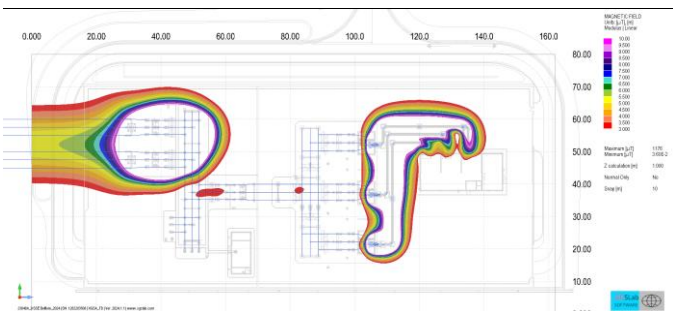
Magnetic field on horizontal surface – Substation – Colors option
