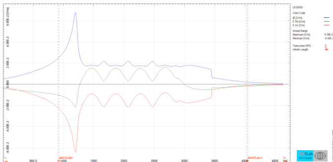
Induced EMF on the pipelines (blue magnitude, green real, red imaginary)
