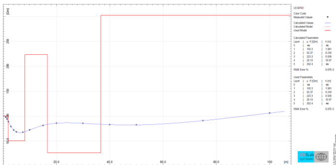
Parameters evaluation for a five layers soil model - Linear scale
