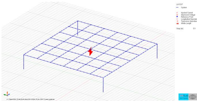
Grounding system layout and current injection point
