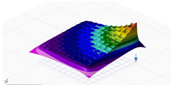
Earth surface potential - GSA_FD with low soil resistivity
