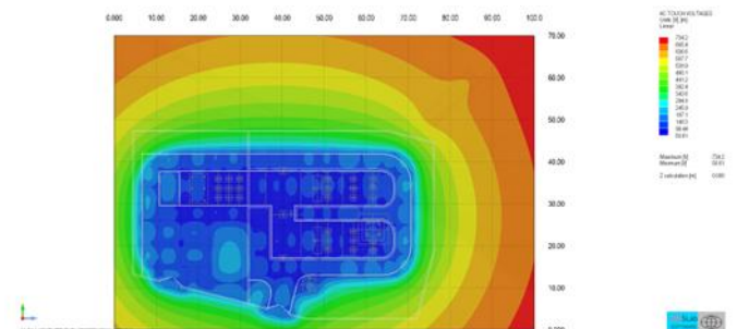
Touch voltages – Substation - Colors option
