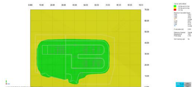
Touch and step voltages safe areas - Substation
