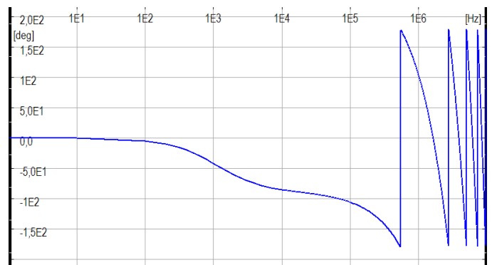
Normalized phase spectrum - Log Linear scale
