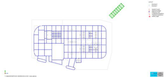
Grounding system layout - Substation
