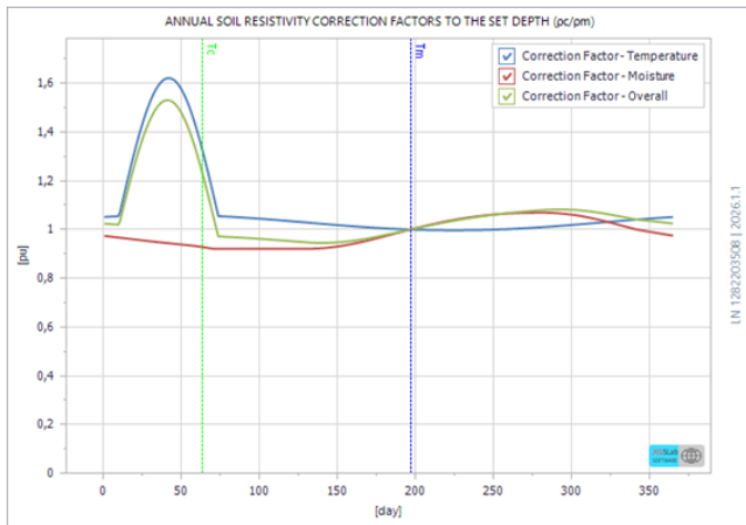
Annual soil resistivity correction factors to the set depth
