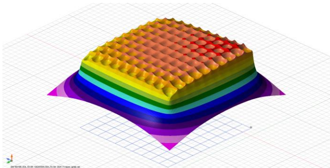
Earth surface potential - 1 kHz
