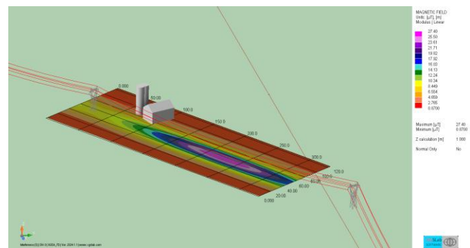
Magnetic field on an horizontal surface – Power line - Colors option
