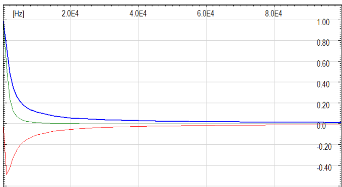
Normalized magnitude spectrum - Magnitude, real and imaginary parts - Linear scale
