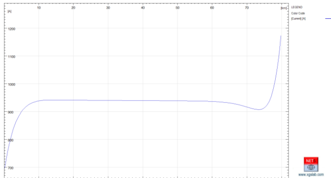
Current along an OHEW – Magnitude - Linear scale
